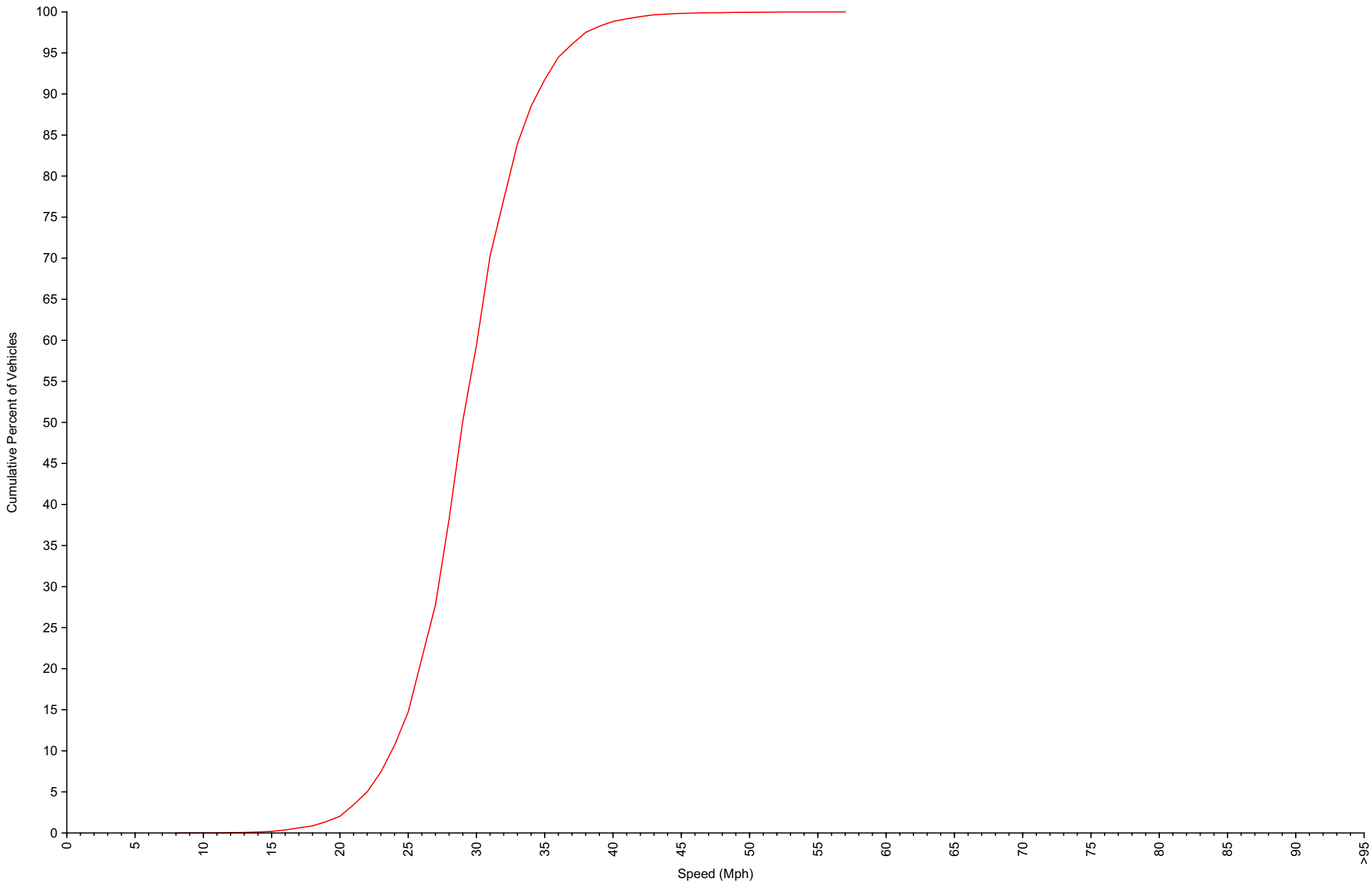
Cumulative Speed Distribution Curve Traffic Overview from Wed Jan 1 2025 to Fri Jan 31 2025
