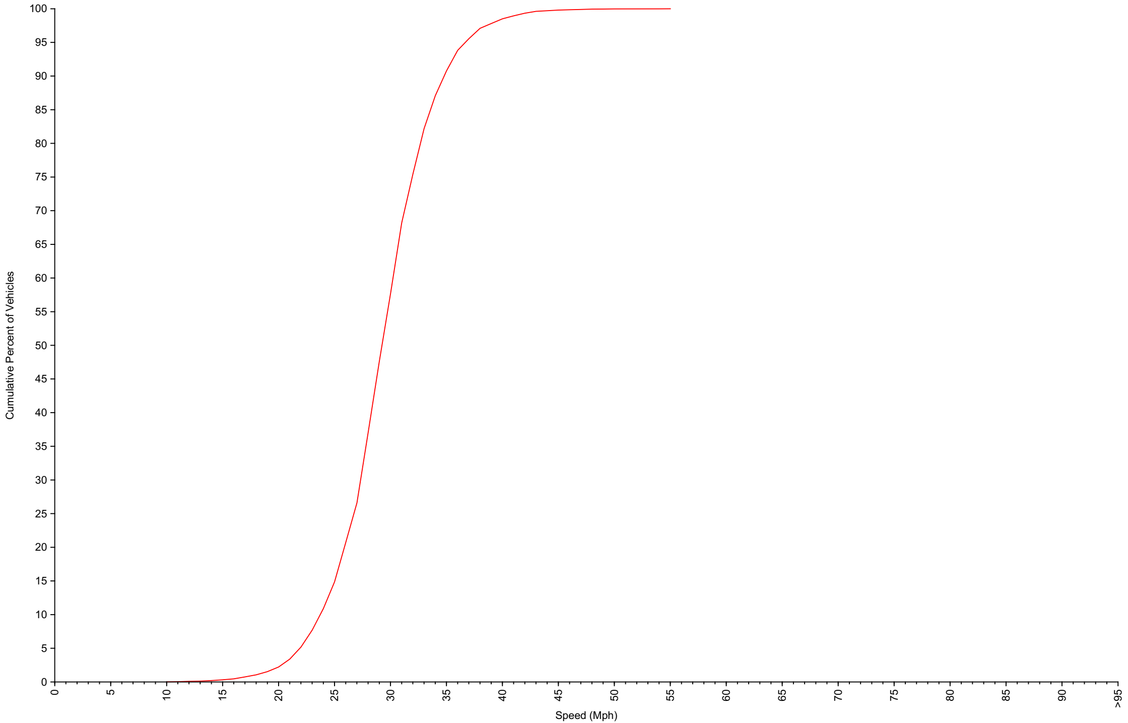
Cumulative Speed Distribution Curve Traffic Overview from Sat Feb 1 2025 to Fri Feb 28 2025
