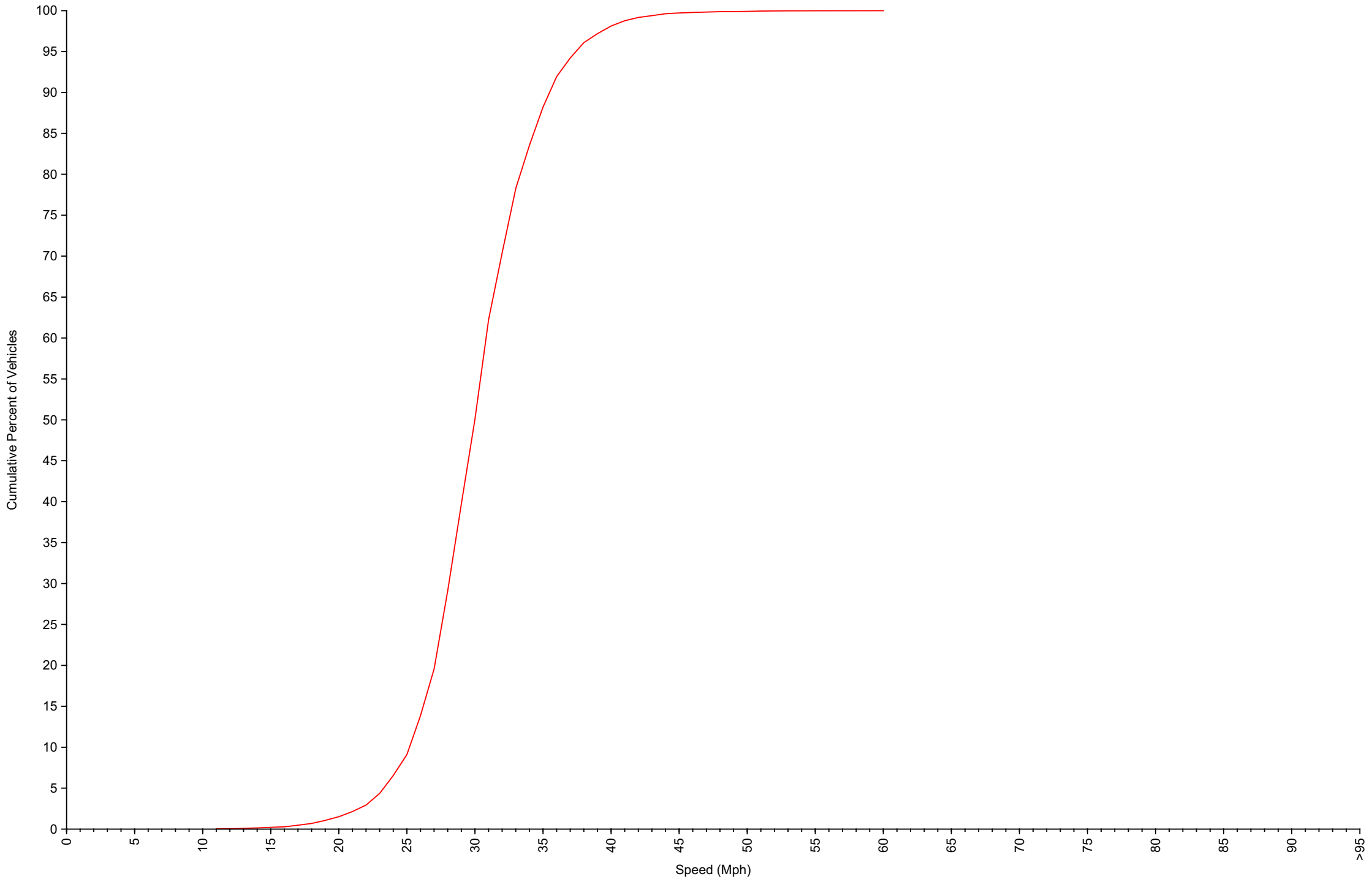
Cumulative Speed Distribution Curve Traffic Overview from Fri Aug 1 2025 to Sun Aug 31 2025
